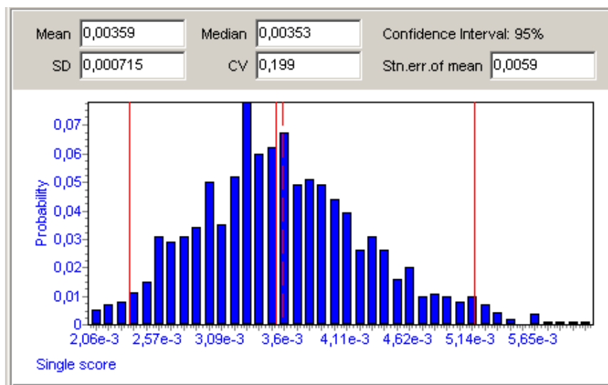
Figure 20 Progress status window during Monte Carlo calculations. Especially the value of the standard error of mean is important to keep track on
