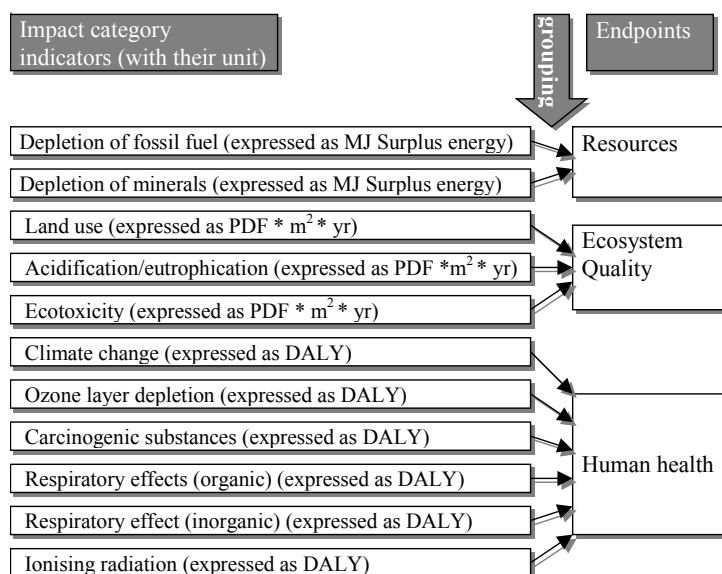
Figure 8 Illustration of the grouping option on the Eco-indicator99 method. This procedure allows to reduce the number of impact categories to just three instead of 11 without subjective weighting
