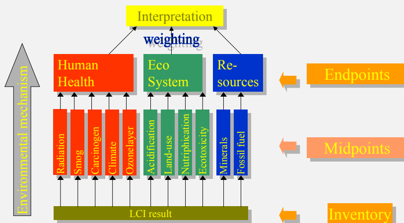
Figure 5 Schematic overview of the methodology proposed by Goedkoop & Spiensma. The environmental models for each impact category are extended up to endpoint level, as the impact category indicators that relate to the same endpoint have a common unit, these indicators can be added. In the case of ecotoxicity, the endpoint is Ecosystem Quality, expressed as Potential Disappeared Fraction of plants
