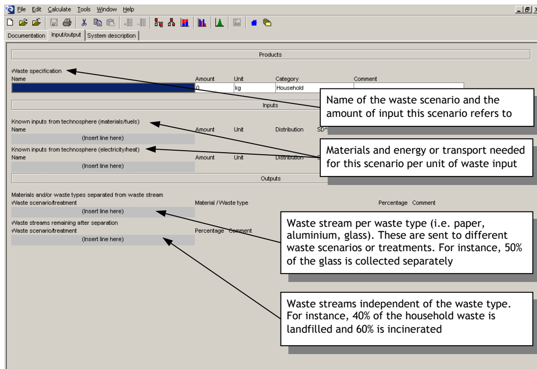
Figure 17 A waste scenario record is used to split a waste stream. Splitting can be done per waste type or in a generic way
