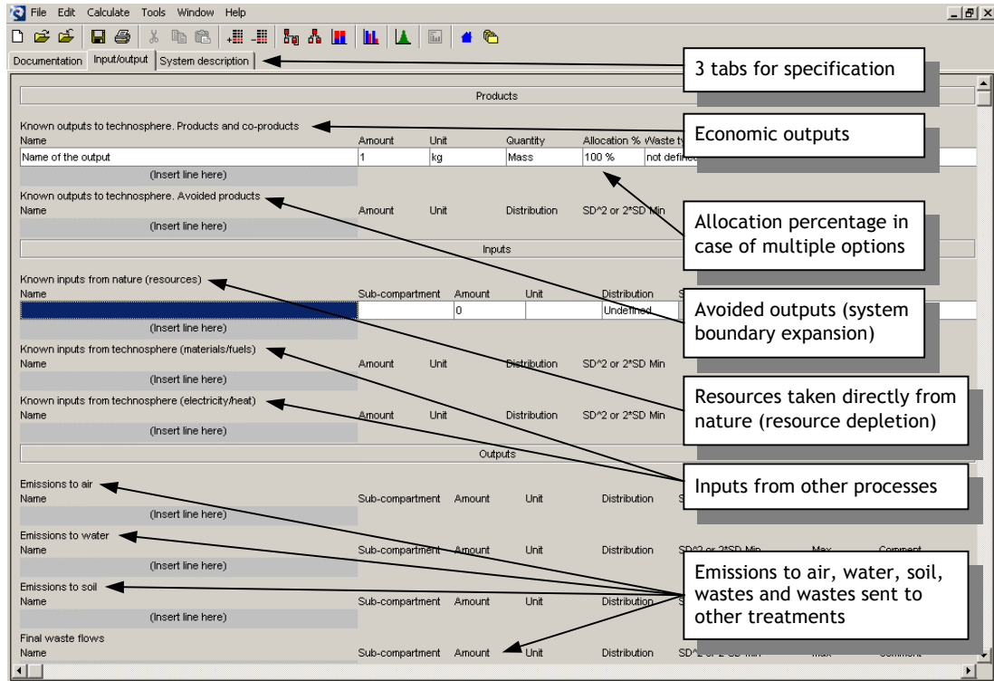
Figure 13: Empty process record (only upper part). This process record is the basic building block for the process tree's in SimaPro
