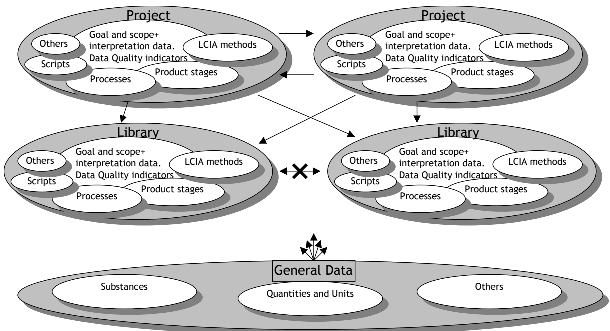
Figure 22 Graphical representation of the database structure. The arrows indicate dependencies. Not all data types are specified, they are referred to as others.
