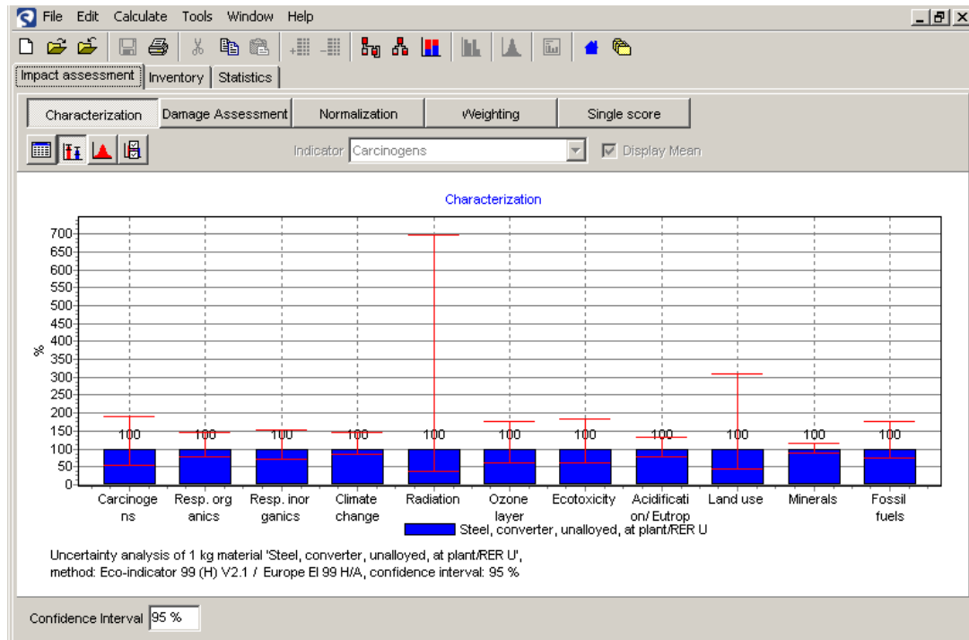
Figure 21 Graphical representation of the Characterization screen for the Converter steel process from the ecoinvent data set. The red lines indicate the 95% confidence intervals. Clearly the score for radiation has a very high uncertainty. Also the uncertainty on the Land-use score is high. The other scores have an uncertainty of about 100%, which is also still very high.
