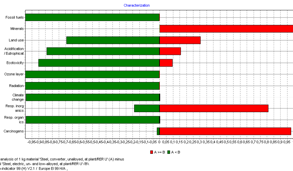
Figure 24 Monte Carlo results of a comparison. In this figure the number of outcomes where converter steel has a higher score than the electro steel are shown per impact category. This allows us to see whether the differences shown in the previous figure are indeed significant. In general we can assume that if 90 to 95% of the Monte Carlo runs are favourable for a product, the difference may be considered significant. Applying this rule means that only the difference between the two processes are not significant for Land use, Acidification and Respiratory inorganic
