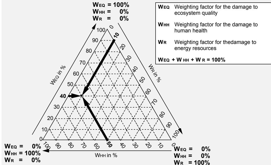
Figure 9: The mixing triangle: The marked weighting point is positioned where Human Health is weighted 50%, Ecosystem Quality 40% and energy Resources 10%. The point is defined by following each side until the dotted flashes leave towards the point in the triangle (based on Hofstetter 1998).
