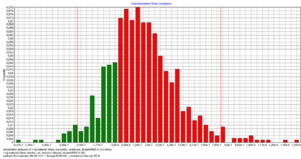
Figure 25 Graphical representation of the difference between Converter and Electro steel during each calculation run. The bars that represent a negative value are plotted in a green colour. A negative value means in this case, Converter steel has a lower score than Electro steel
