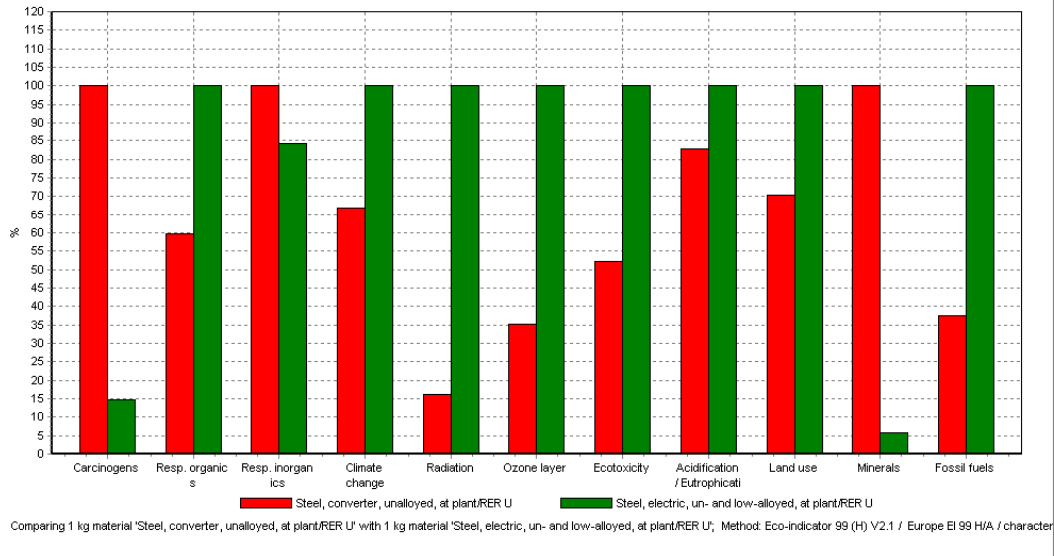
Figure 23 Standard comparison between two ways of producing steel. We see that Electro steel has a lower impact on Carcinogens, Respiratory Inorganic and Minerals
